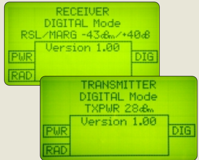
DAR Plus Front Panel Display (Transmitter & Receiver)
